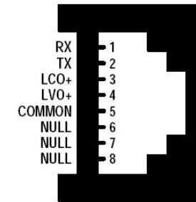
Fig1: RJ45 Interface (Side view)
