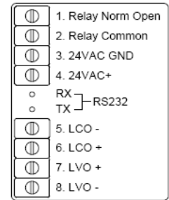
Fig 2: Wiring Connection
